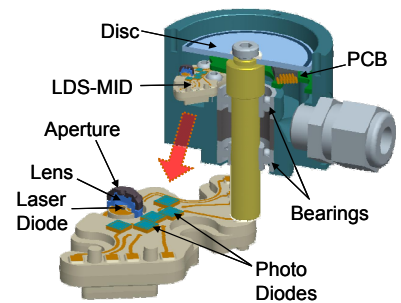
Fig. 4: Low cost assembly concept using MID-Technology
