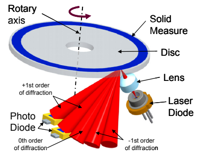
Fig. 2: Optical reading unit of an incremental angular resolver
