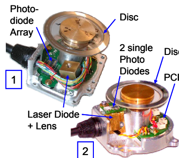
Fig. 3: Absolute encoded (1) & incremental (2) resolver
